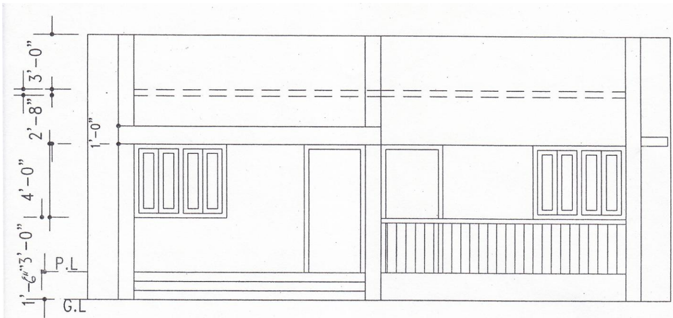
FRONT ELEVATION
